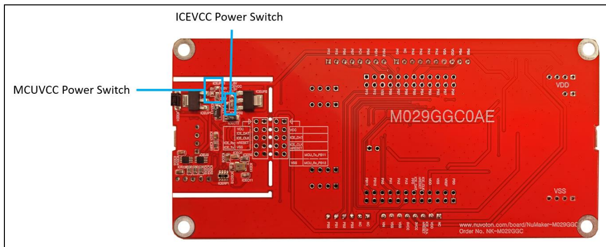
Figure 3-2 Rear View of NuMaker-M029GGC
