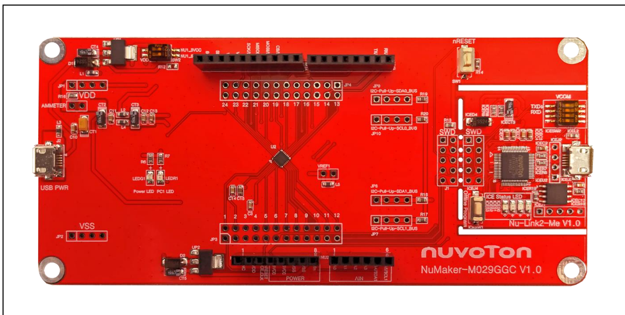
Figure 1-1 NuMaker-M029GGC Evaluation Board
