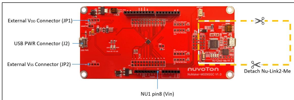
Figure 3-7 Detach the Nu-Link2-Me from NuMaker-M029GGC
