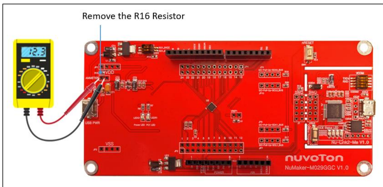
Figure 3-8 Wiring between Ammeter Connector and Ammeter
