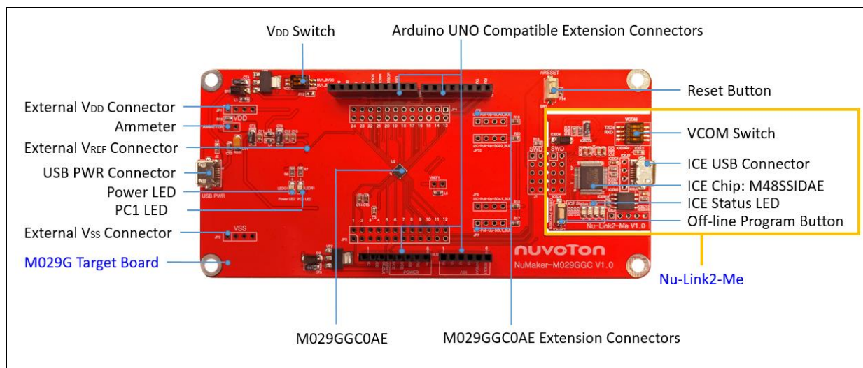
Figure 3-1 Front View of NuMaker-M029GGC
