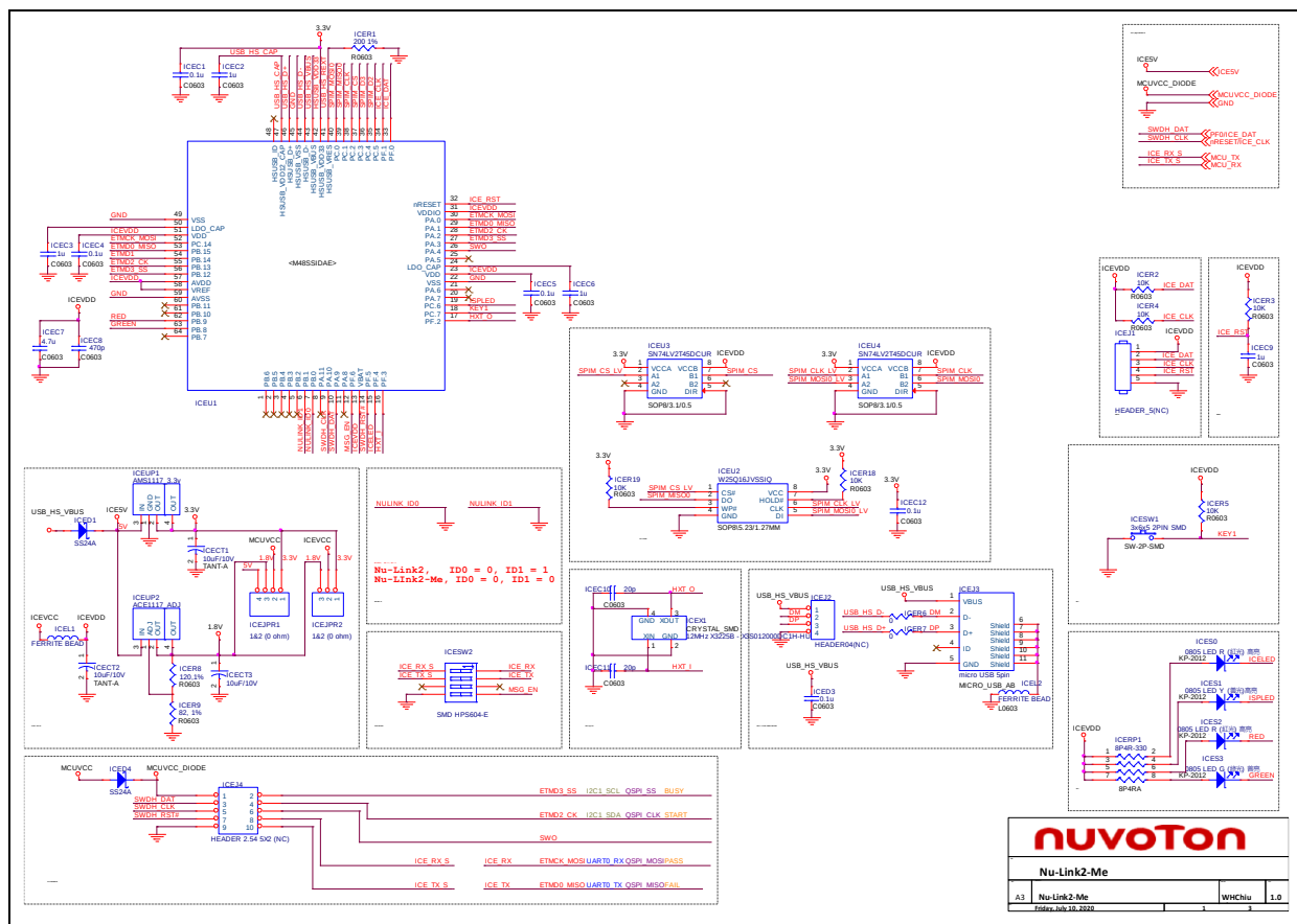
Figure 5-1 Nu-Link2-Me Circuit
