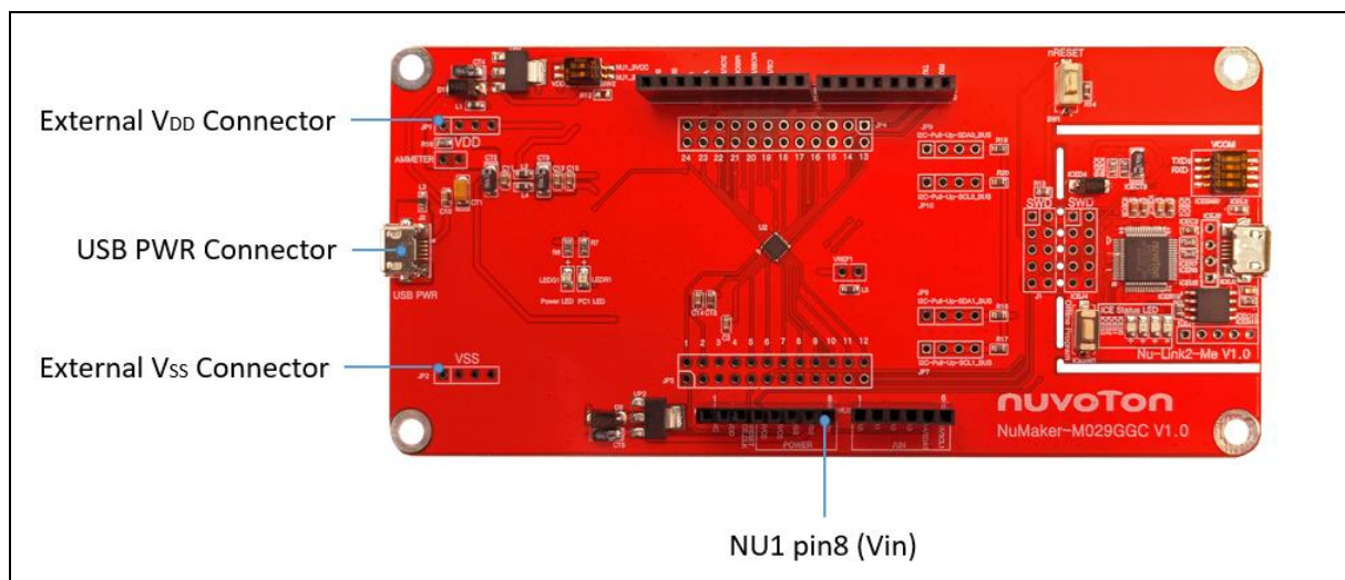
Figure 3-6 External Power Supply Sources on M029GGC Target Board
