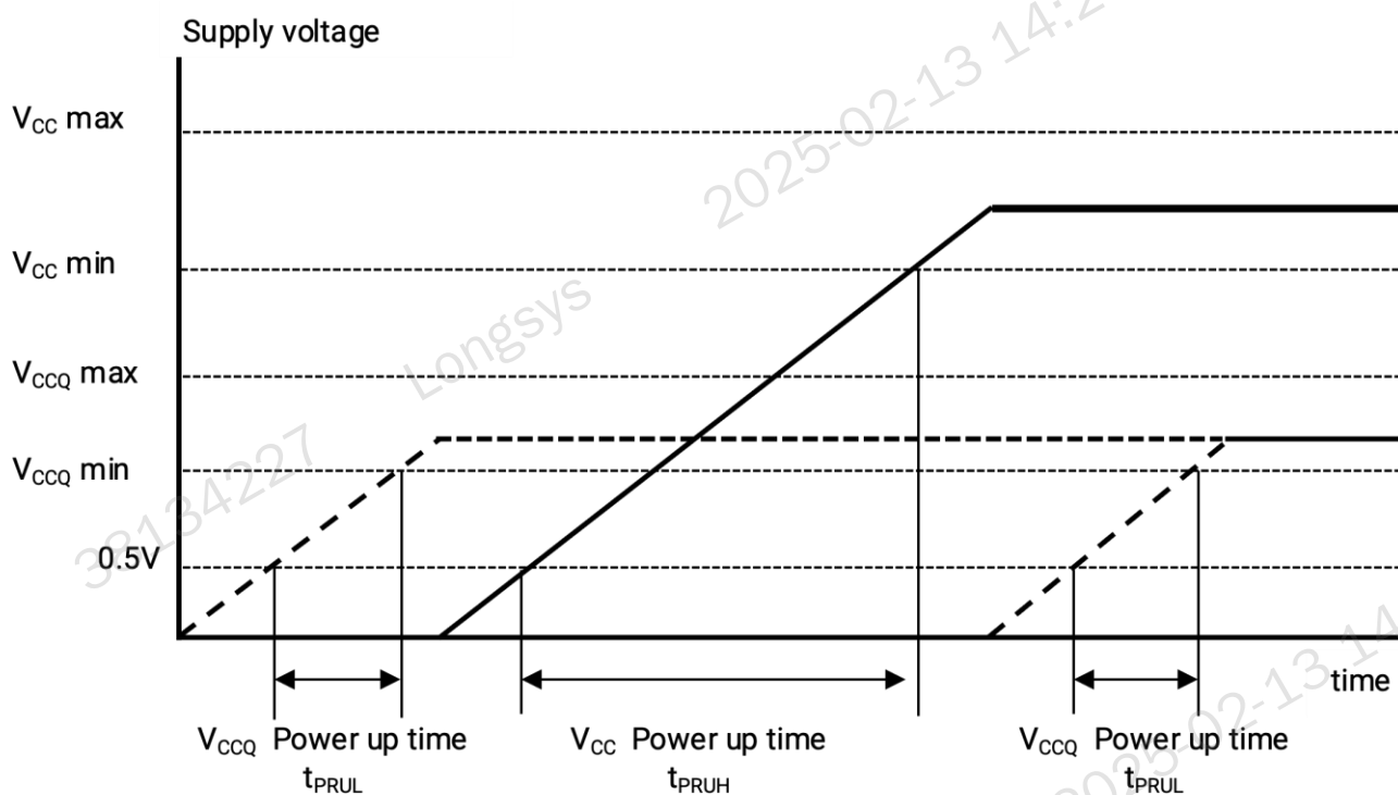
Figure 15 Power-on Sequence
