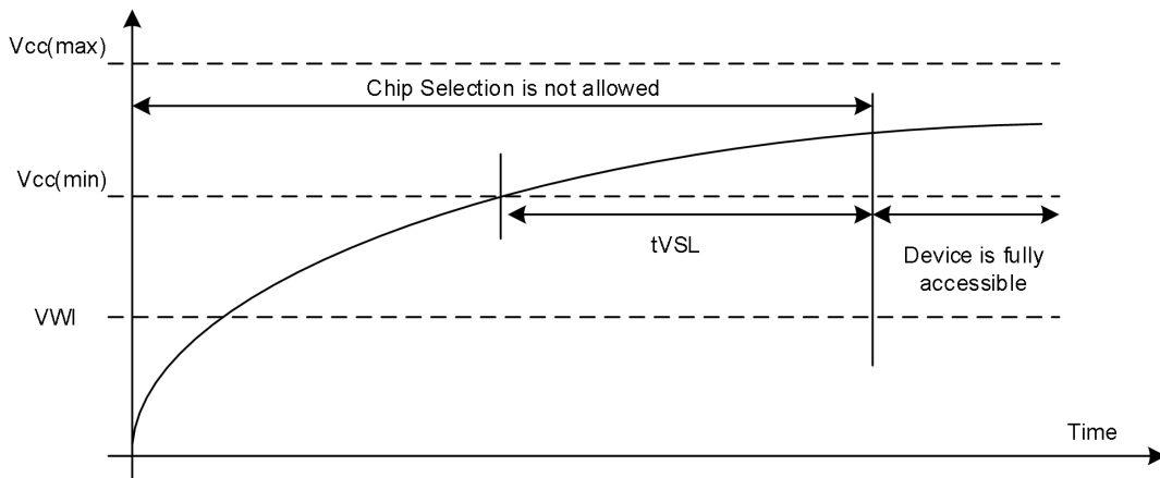
Figure26. Power-On Timing
