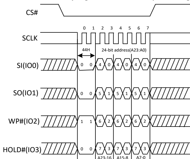
Note: The device default is in 24-bit address mode. For 4-byte mode, the address length becomes 32-bit.
