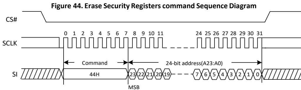
Note: The device default is in 24-bit address mode. For 4-byte mode, the address length becomes 32-bit.
