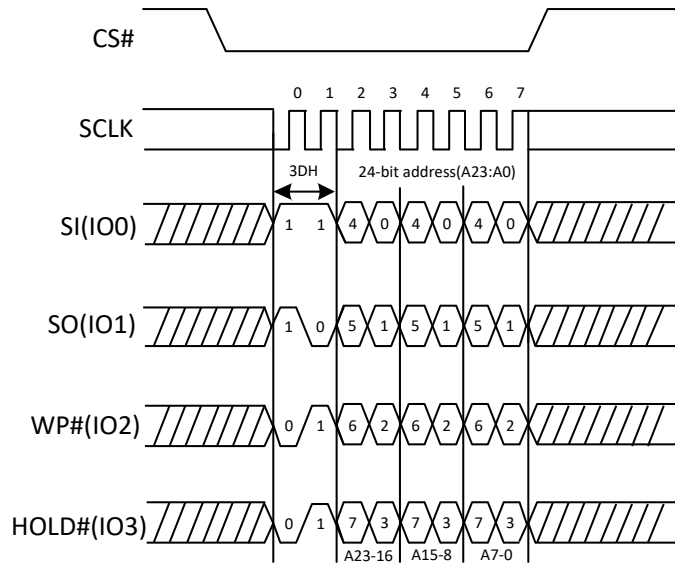
Figure 46e. Read Individual Block/Sector lock command Sequence Diagram (QPI)
