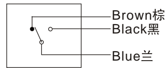
Output CO(NO+NC)
